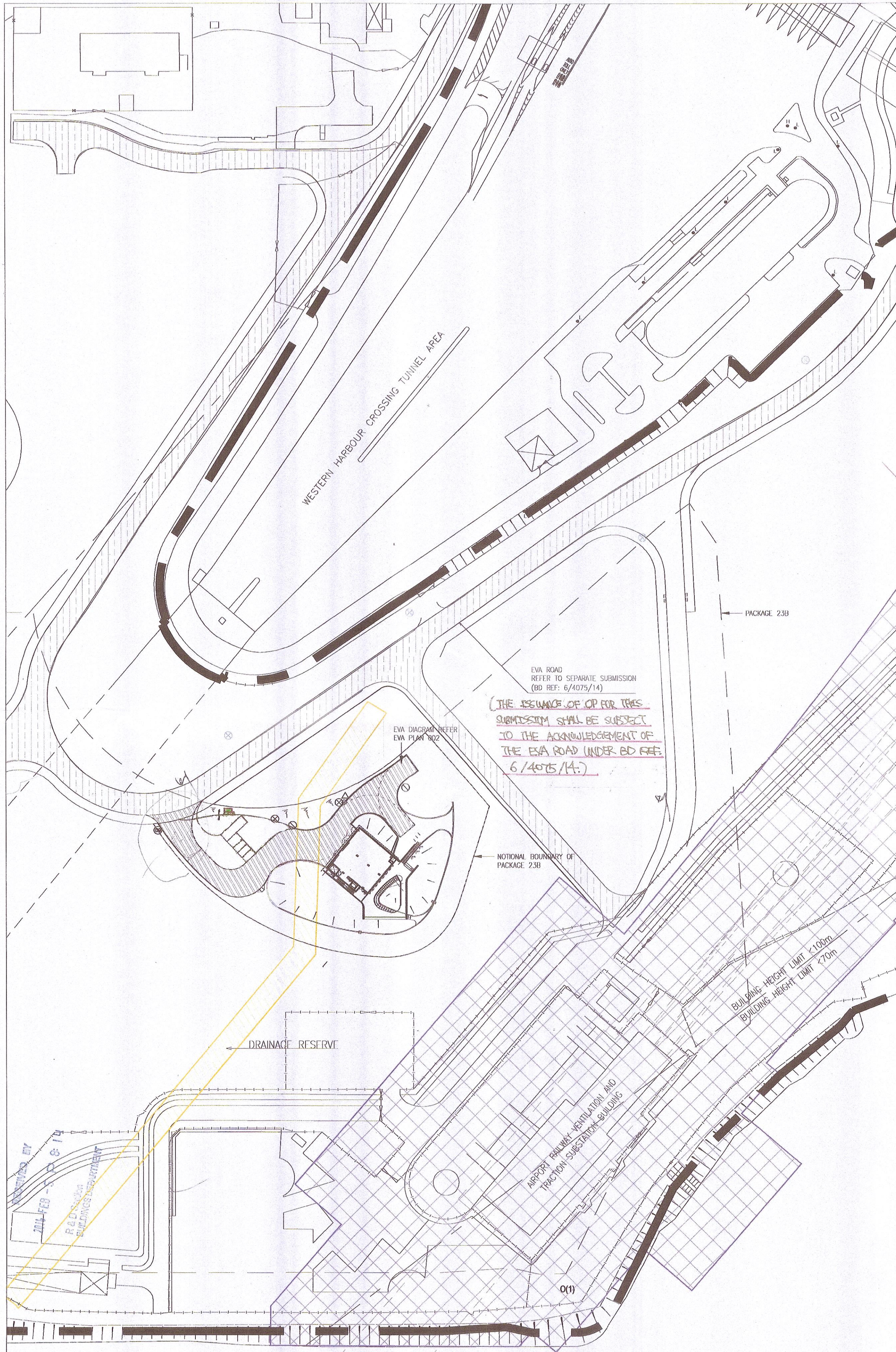
001 MASTER LAYOUT PLAN SCALE 1:1000
